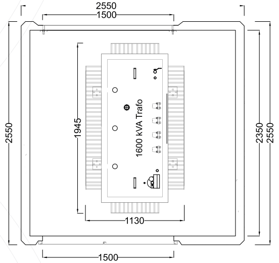
MBK 2500/1600
